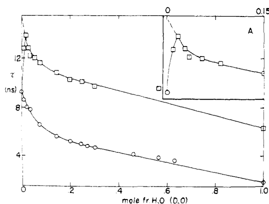
FIGURE 2: Variation in ethidium bromide fluorescence lifetime in acetone solution as a function of added H 2 O (○) or D 2 O (□). Dashed curve represents extrapolation of deuterated ethidium bromide lifetime to zero mole fraction D 2 O. Inset A shows the effect of small amounts of added D 2 O on an expanded mole-fraction scale.
